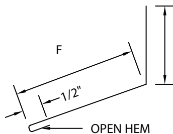
COUNTER FLASHING
