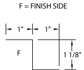
ZEE CLOSURE
