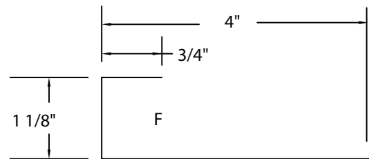
CHANNEL CLOSURE
