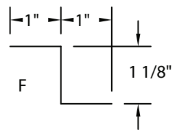
ZEE CLOSURE
