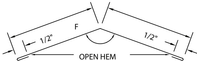
HIP FLASHING
