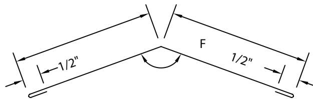
RIDGE FLASHING
