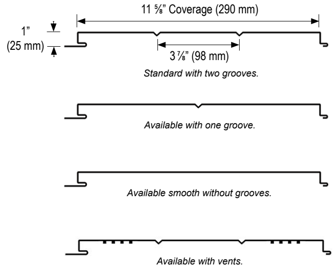
Berridge L-Panel is an economical and versatile panel for fascia, soffit, liner and ceiling applications. Available with 2 grooves, 1 groove or no grooves as shown above.
