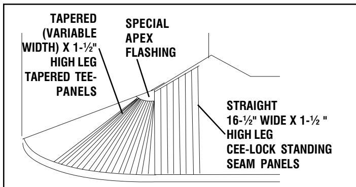
FIG. 2 - Leg heights of the Berridge Cee-Lock and Tapered High Seam Tee-Panel match up perfectly for a smooth transition.
