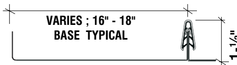
FIG. 3 - The seam configuration of Berridge High Seam Tee-Panel matches that of the Berridge Cee-Lock panel (below, FIG. 4)
