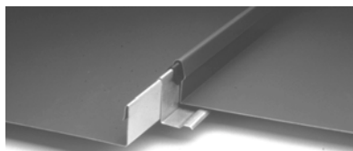
FIG. 4 - Berridge Cee-Lock, with its integral snap lock seam and 16-1/2" wide coverage is an aesthetic, economical roof panel.
