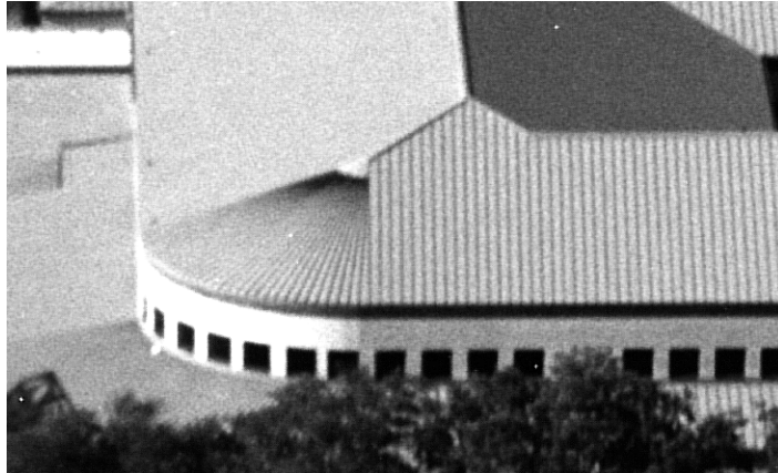
FIG. 1 - A smooth transition from straight Berridge Cee-Lock standing seam panels to tapered Berridge Tapered High Seam Tee-Panels provides an eye-pleasing rounded corner roof design.
